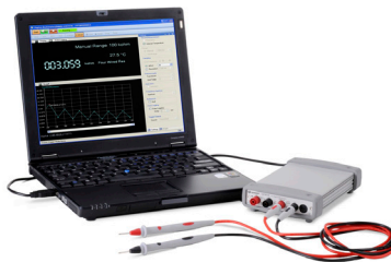
U2741A used as a standalone instrument
